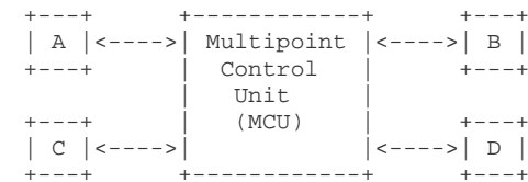
Figure 8 - Point to Multipoint Using Content Modifying MCUs
