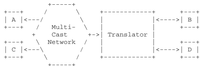
Figure 3 - Point to Multipoint Using a Translator
